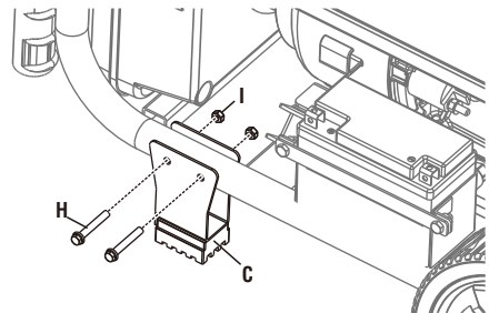
Pied de support ×2
