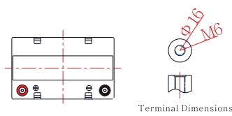
Terminal Dimensions
